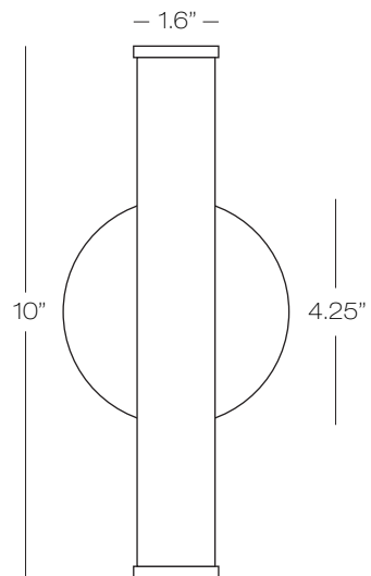
Wall projection 3"
